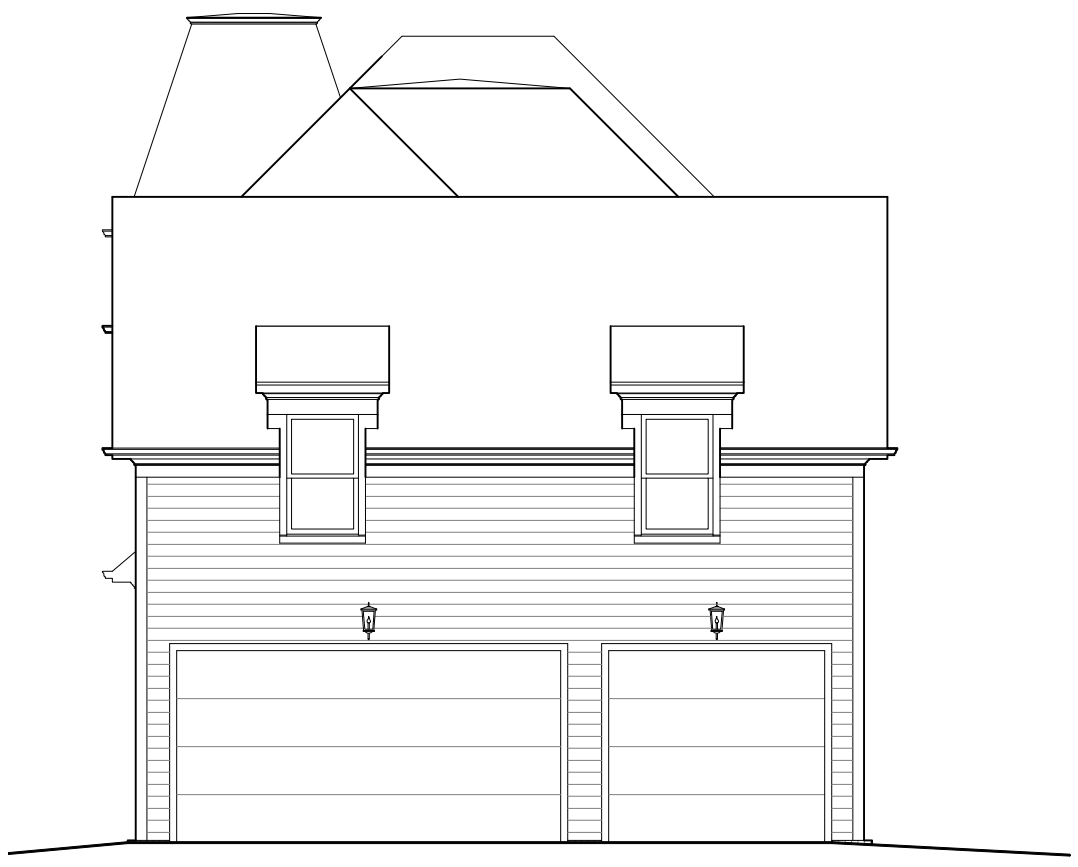
2 REAR ELEVATION 1/8" = 1'-0"
