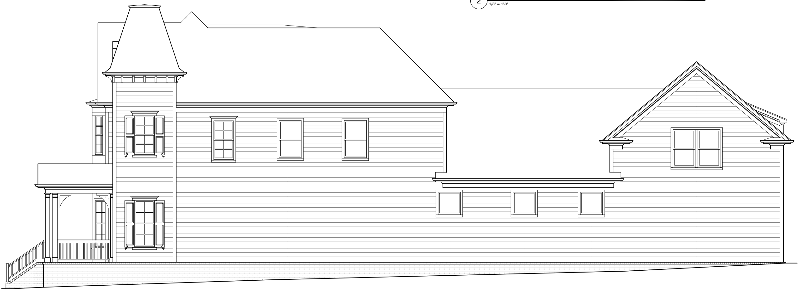
1 LEFT ELEVATION 1/8" = 1'-0"
